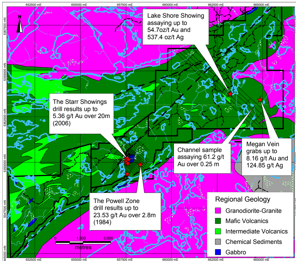
Figure 2: Regional geology map of Saganaga/Q9 property with highlights.
